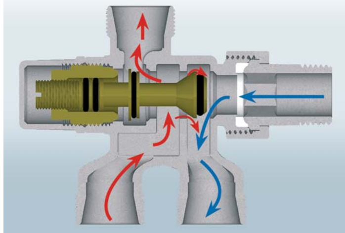
Flow circulation inside the valve
