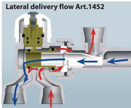
Example of installation of Art.1452
